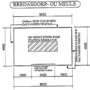
:LAYOUT PLAN :DRAWING SCALE 1:100
