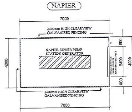
:LAYOUT PLAN :DRAWING SCALE 1:100
